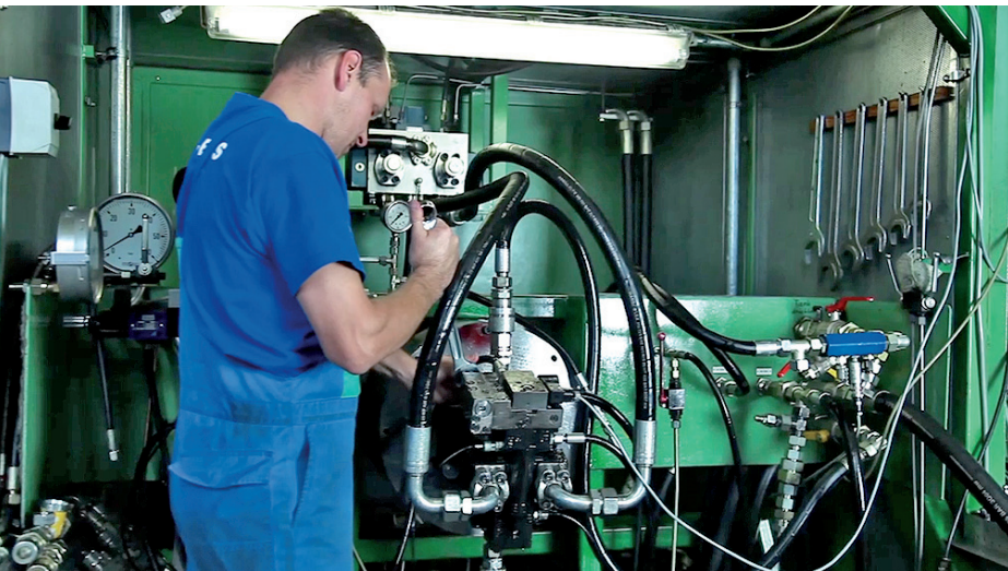
Test benches for open and closed circuit
