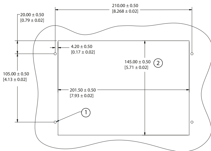
Panel cutout (mm [in]) and panel mounting spring clip
