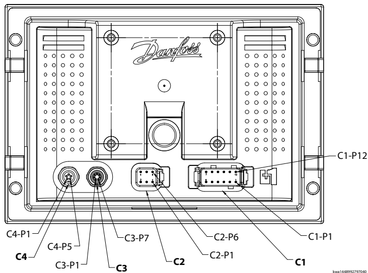
DP6XX series, pin assignments
