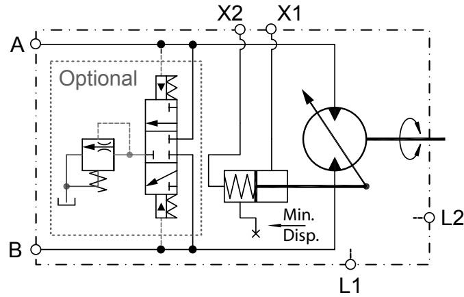
SAE motor - single or two line control
