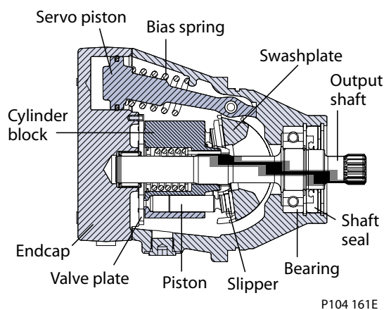
Cross section, cartridge mount
