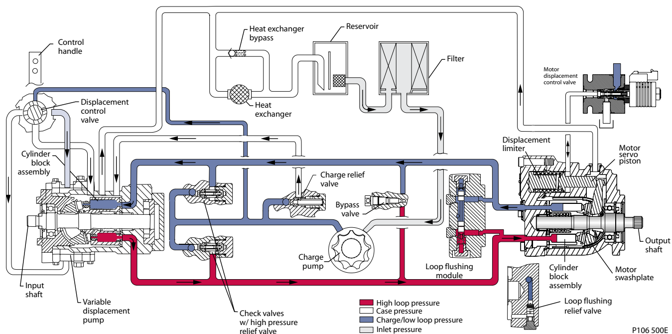
Pictorial system diagram
