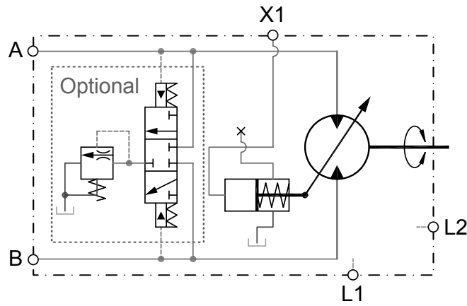
Cartridge motor - single line control
