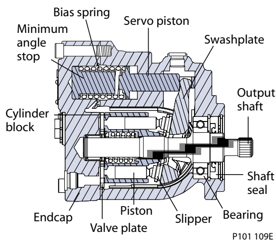
Cross section, cartridge mount
