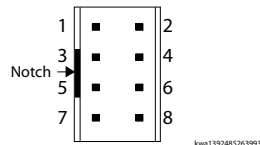
Pinout and wiring information
