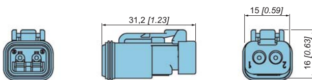
Socket contact
